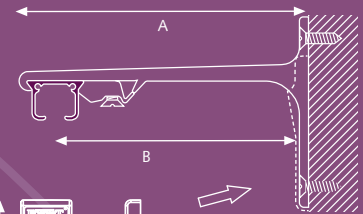
Smart Klick Cover Cap Alu Wall Bracket Universal
